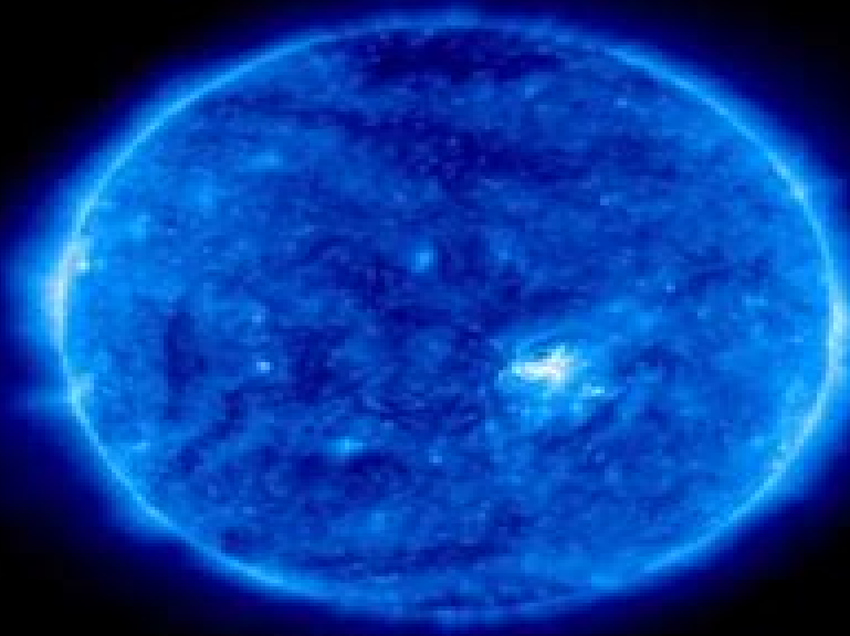
Fe IX, X, 171 Angstroms
